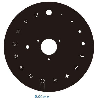
VIZI BEAM I2RX GOBO WHEEL
