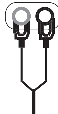
Typical speaker output using spade connectors. Insert bare wire into the binding post and tighten.
