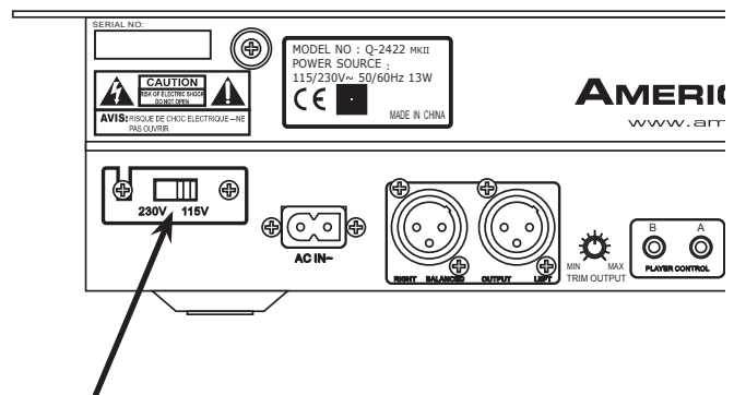
VOLTAGE SELECTOR SWITCH
