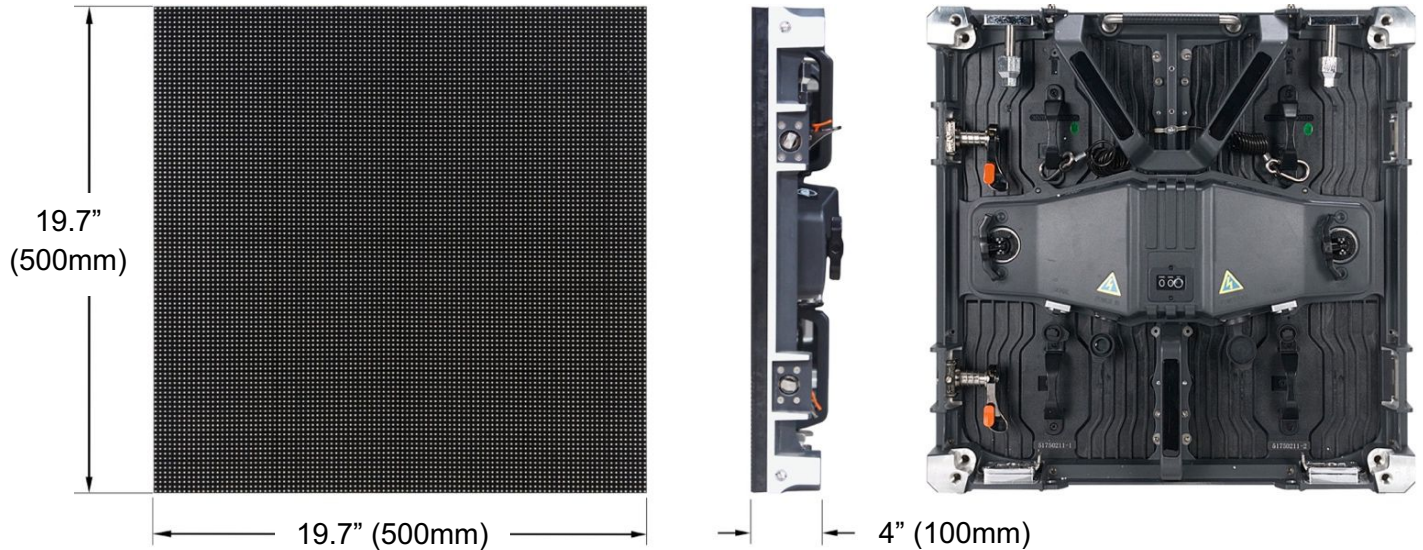
AV4XIP: Front, Side, & Back View
