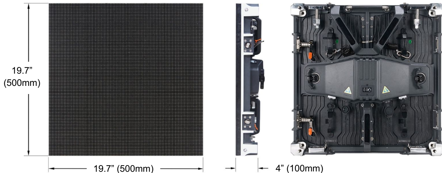
AV4IP: Front, Side, & Back View
