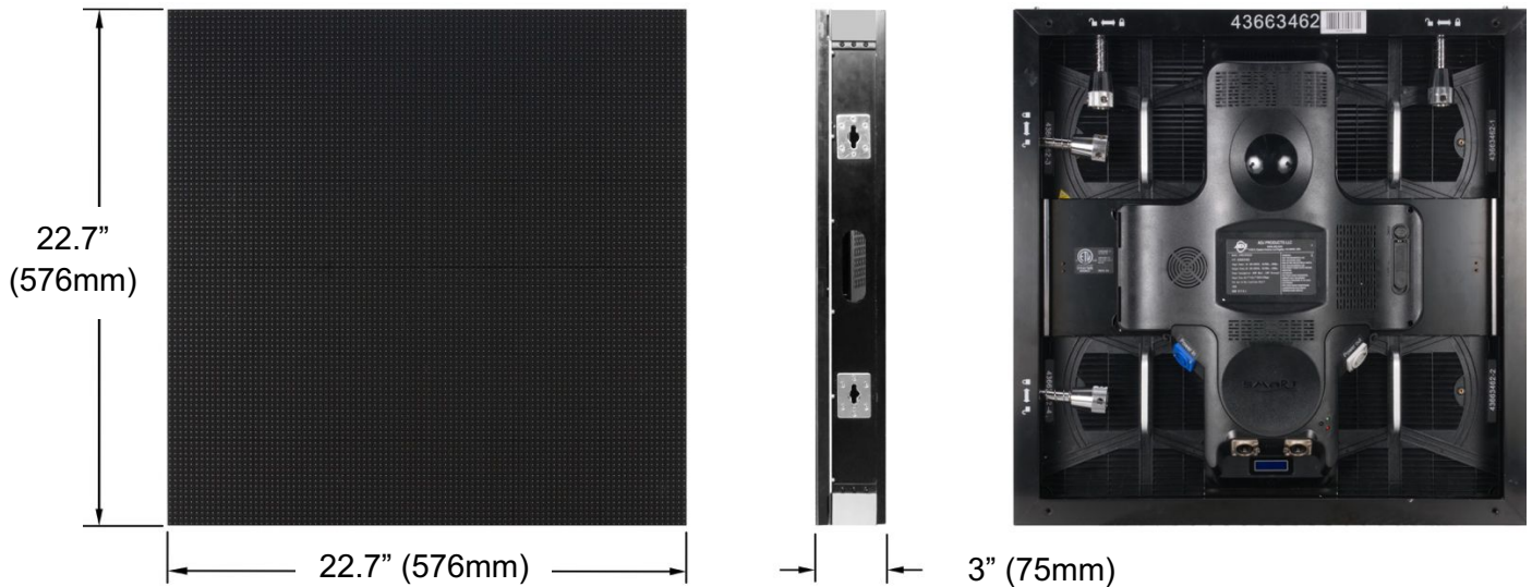
AV6X: Front, Side, & Back View
